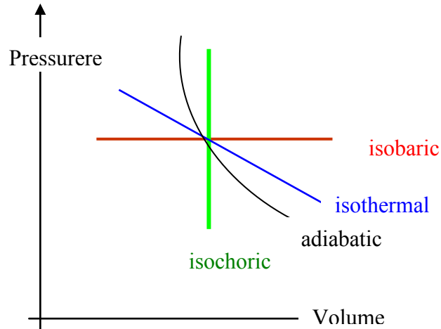
Figure 2.1: Process paths
