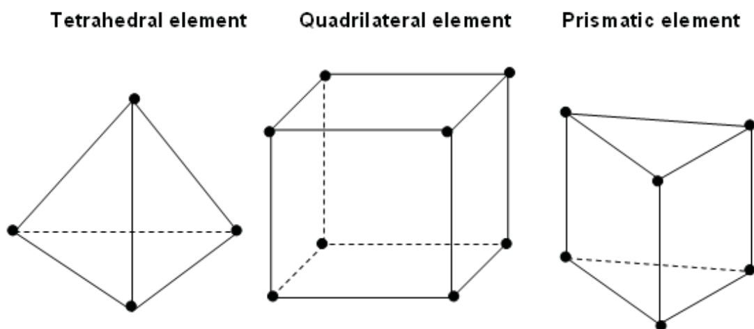
Figure 6-11: Three-dimensional elements
